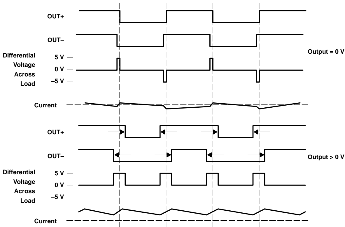
Figure 29. The TPA2000D4 Output Voltage and Current Waveforms Into an Inductive Load
