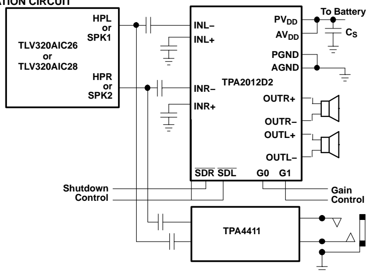
APPLICATION CIRCUIT
