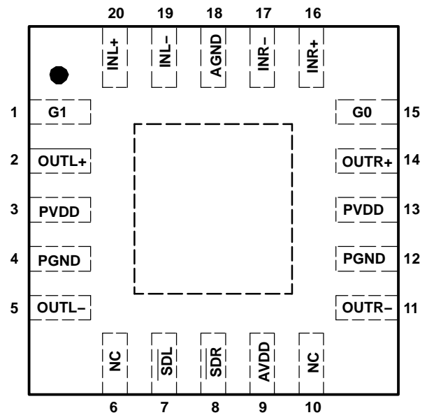
RTJ PIN OUT TOP VIEW
