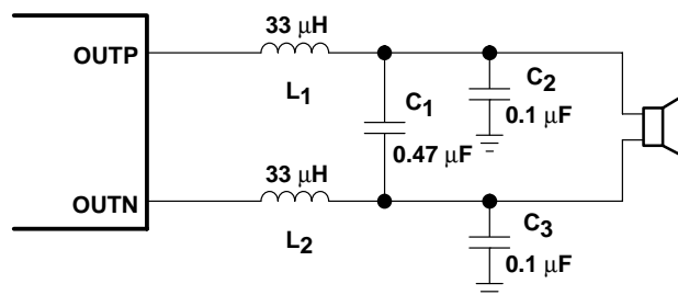
Figure 33. Typical LC Output Filter, Cutoff Frequency of 41 kHz, Speaker Impedance = 8 \Omega
