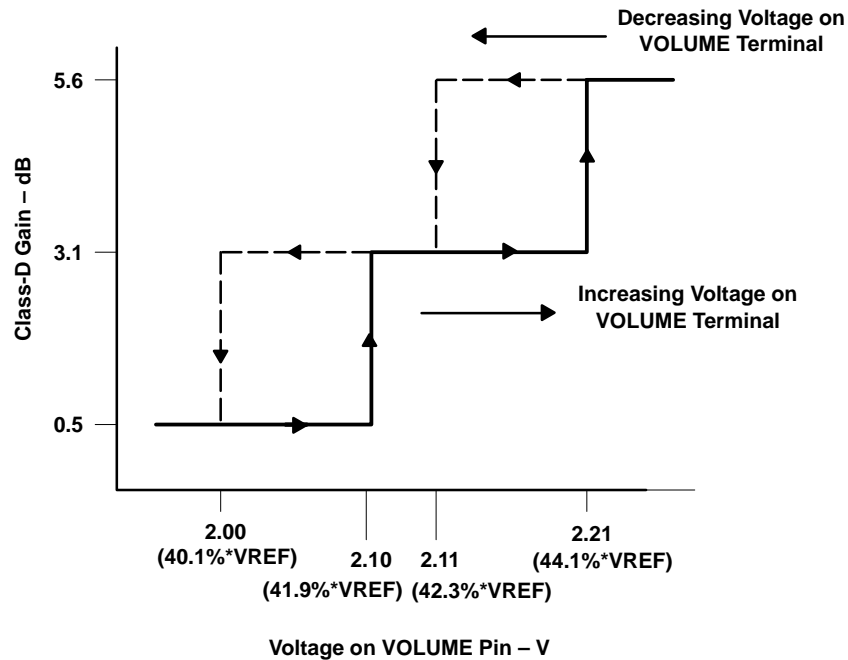
Figure 36. DC Volume Control Operation, VREF = 5 V
