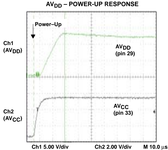
Figure 37. Power-Up Response
