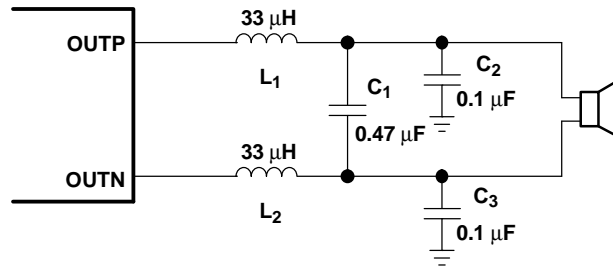
Figure 18. Typical LC Output Filter, Cutoff Frequency of 27 kHz, Speaker Impedance = 8 Ω
