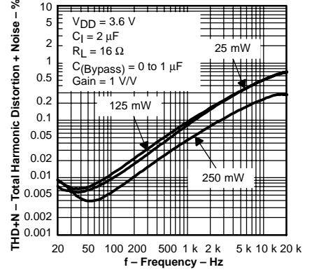
TOTAL HARMONIC DISTORTION + NOISE vs FREQUENCY
