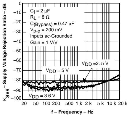
SUPPLY VOLTAGE REJECTION RATIO vs FREQUENCY
