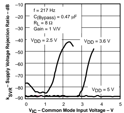
SUPPLY VOLTAGE REJECTION RATIO vs COMMON-MODE INPUT VOLTAGE
