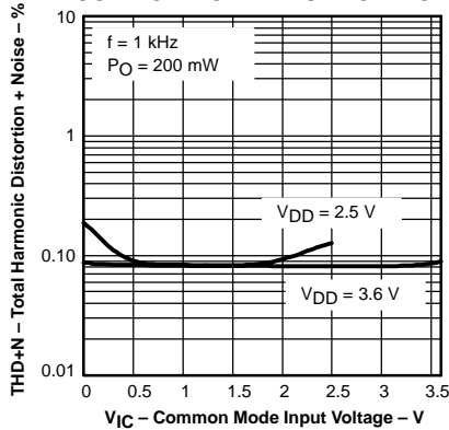
TOTAL HARMONIC DISTORTION + NOISE vs COMMON MODE INPUT VOLTAGE
