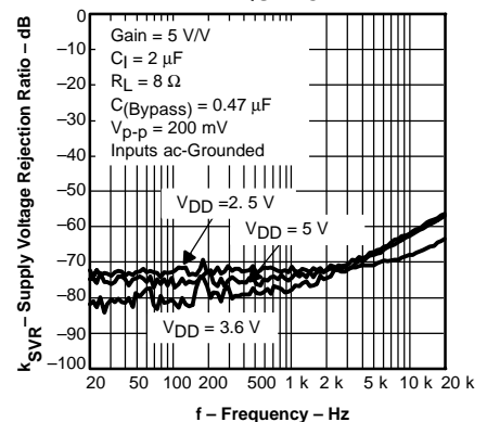
SUPPLY VOLTAGE REJECTION RATIO vs FREQUENCY
