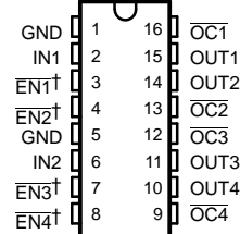
TPS2044B/TPS2054B D PACKAGE (TOP VIEW)
