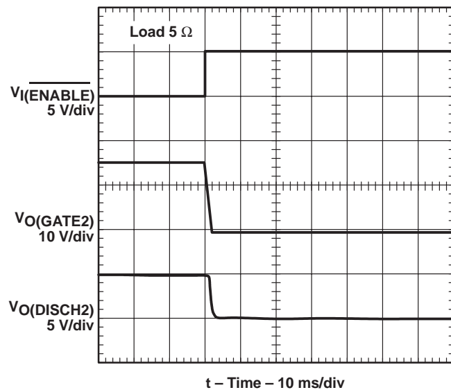
Figure 4. Turnoff Voltage Transition of Channel 2
