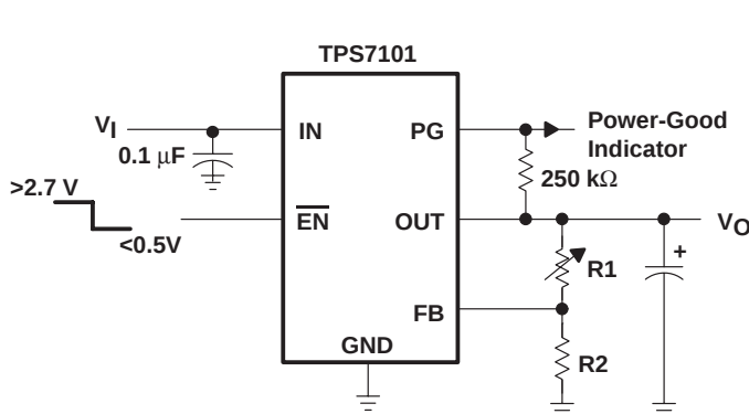
Figure 44. TPS7101 Adjustable LDO Regulator Programming
