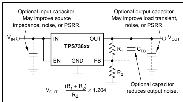
Figure 32. Typical Application Circuit for Fixed-Voltage Versions
