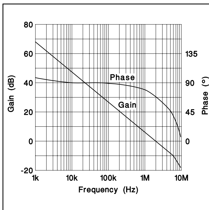
Figure 2. Error amplifier gain/phase response.
