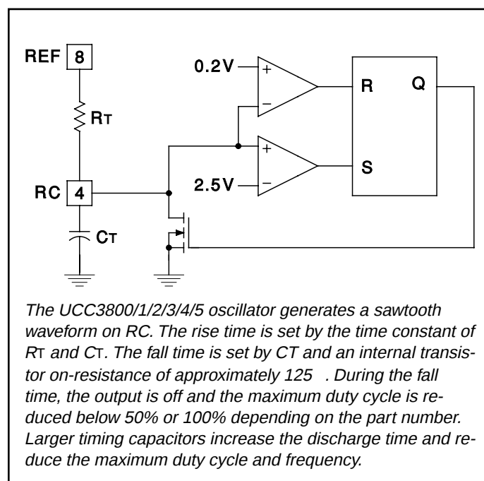
Figure 1. Oscillator.
