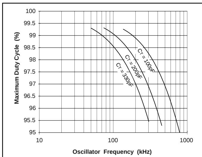
Figure 6. UCC1800/2/3 maximum duty cycle vs. oscillator frequency.
