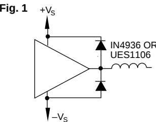
Fig. 1 PROTECTION, INDUCTIVE LOAD
