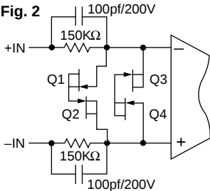
Fig. 2 PROTECTION, OVERVOLTAGE
