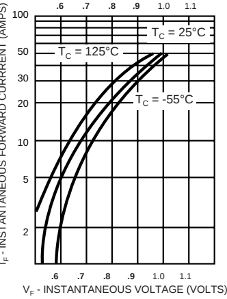
TYPICAL FORWARD VOLTAGE OM4215SA
