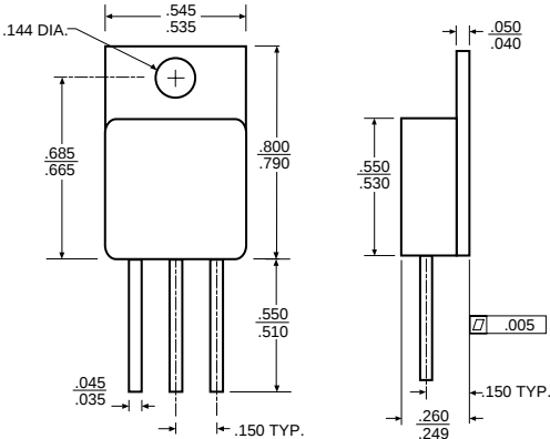
MECHANICAL OUTLINE
