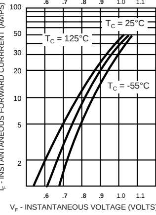
TYPICAL FORWARD VOLTAGE OM4216SA
