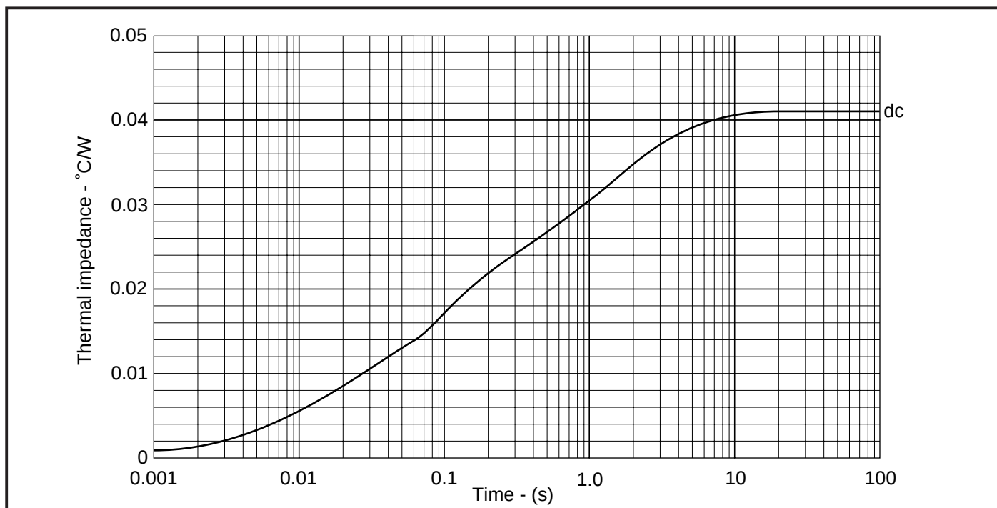
Fig.4 Maximum (limit) transient thermal impedance - double side cooled
