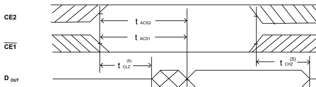
READ CYCLE2 (1,3,4)
