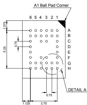
BOTTOM VIEW ( BALL SIDE )
