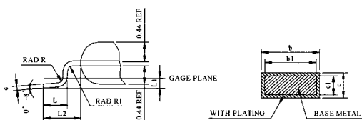
SECTION Y-Y
