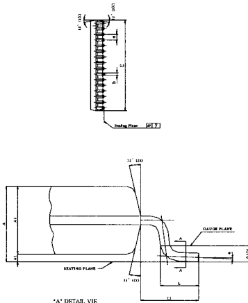
'A' DETAIL VIE
