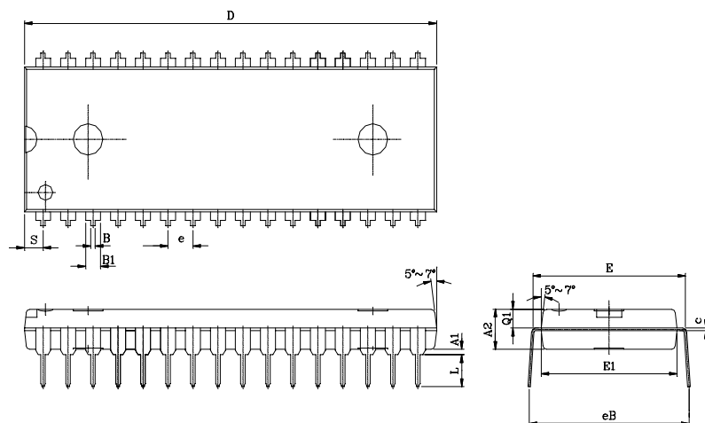
PDIP - 32
