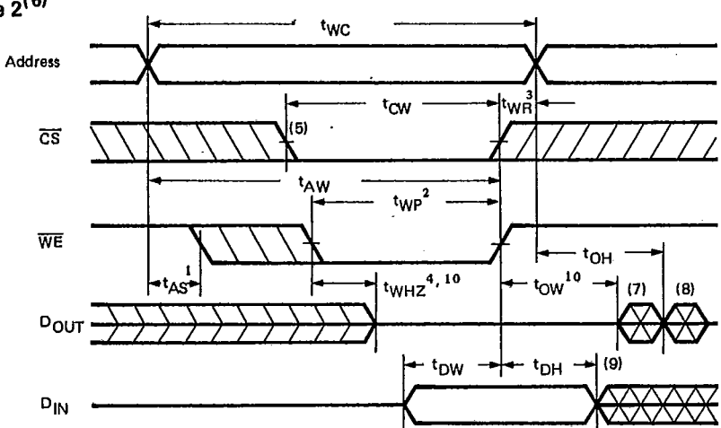
Write Cycle 2 (6)
