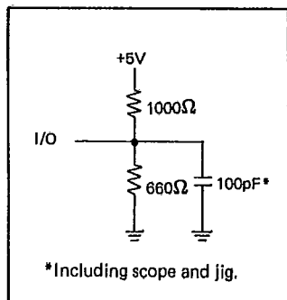
Figure 1. Output Load
