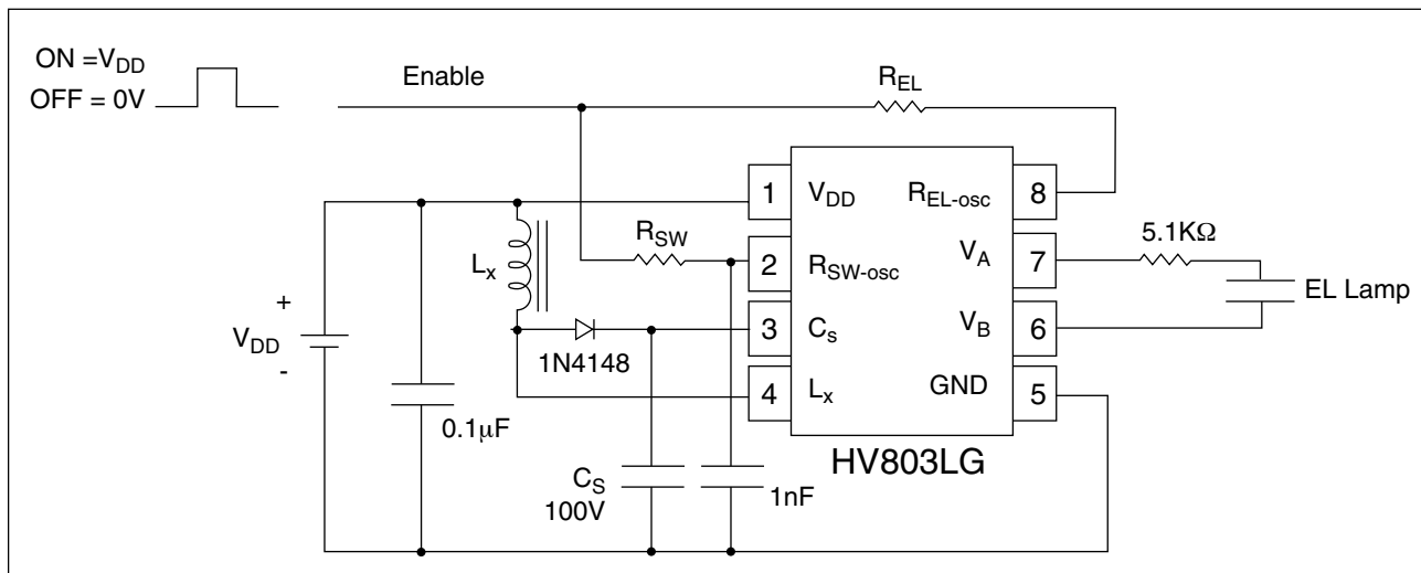
Figure 4: Enable/Disable Configuration
