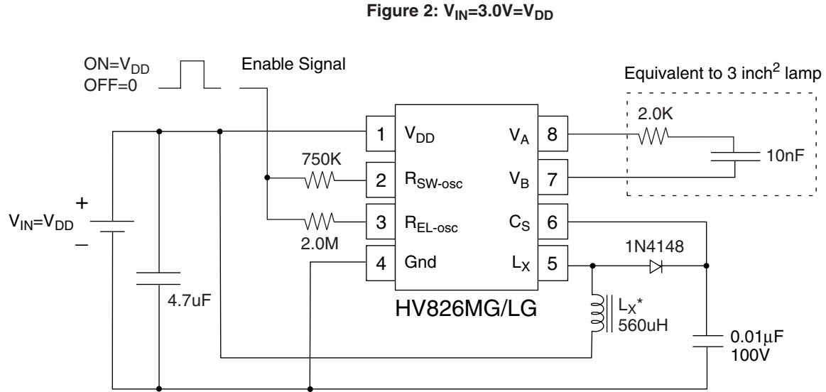
Figure 2: Typical Application
