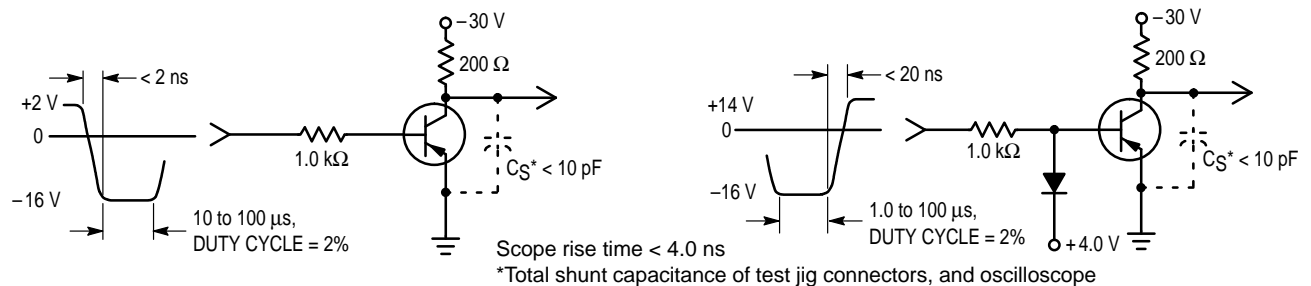
Figure 1. Turn–On Time
