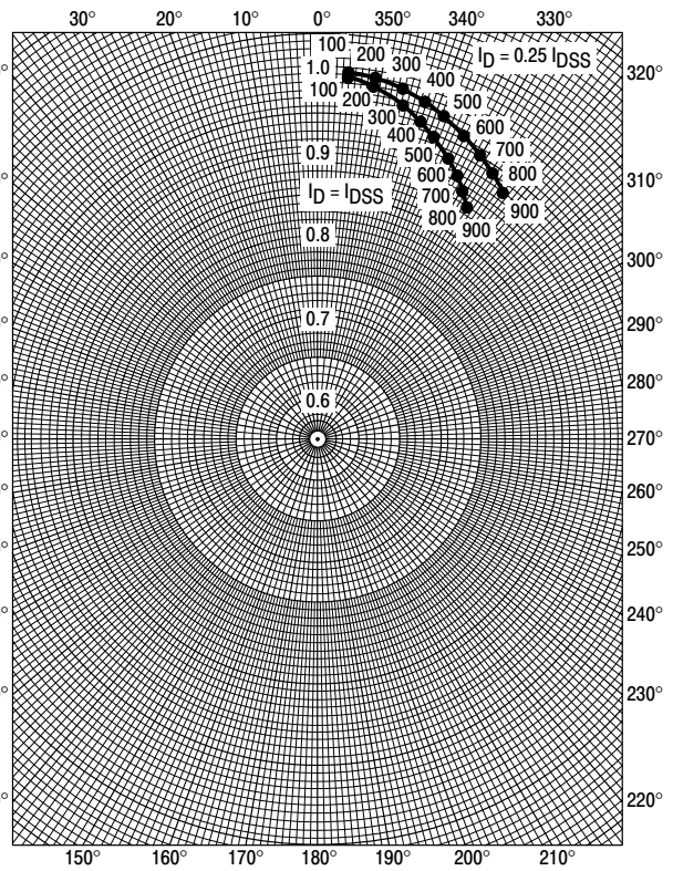
Figure 8. S_{22s}
