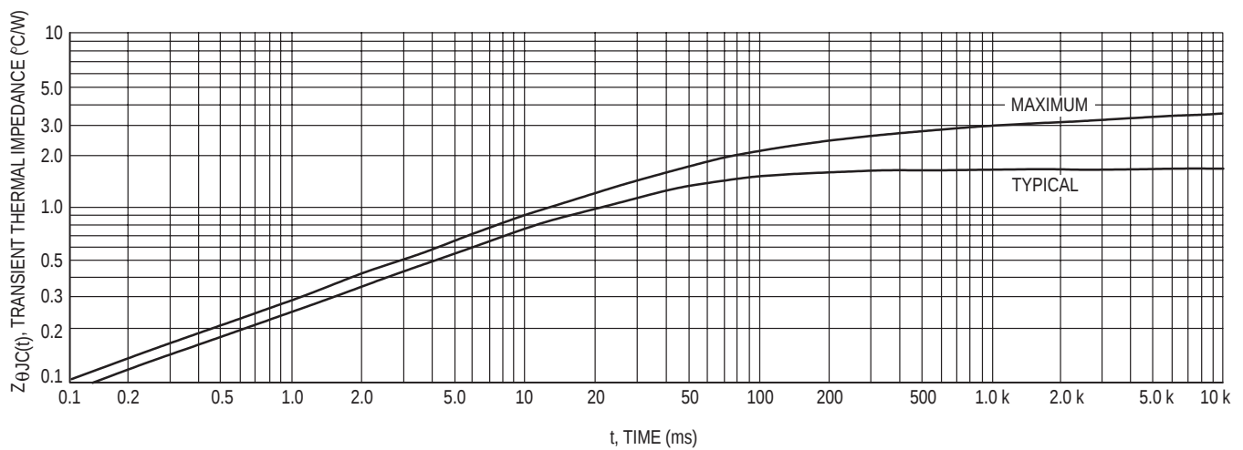
Figure 10. Thermal Response
