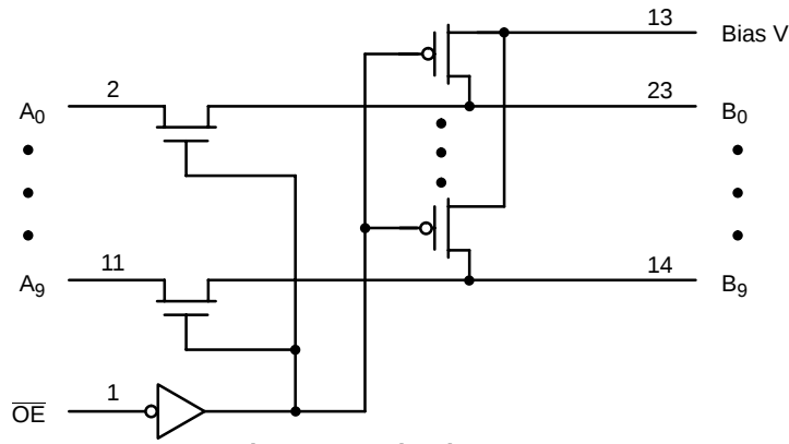
Figure 2. Logic Diagram
