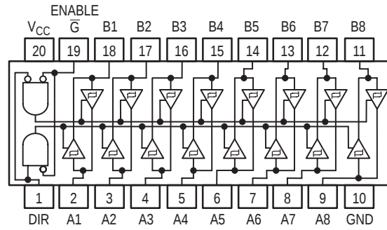
SN74LS641 SN74LS645
