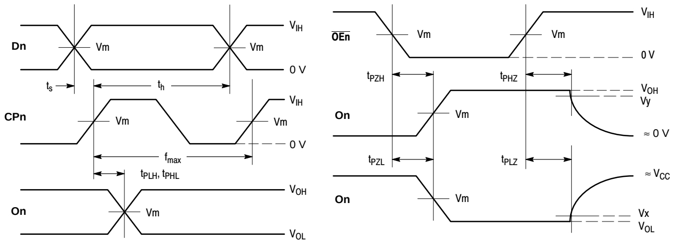
Figure 4. AC Waveforms
