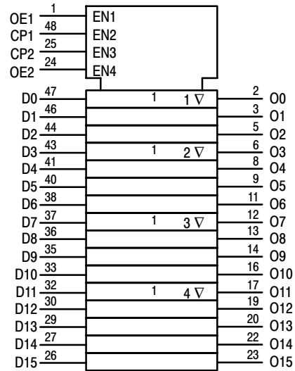
Figure 3. IEC Logic Diagram
