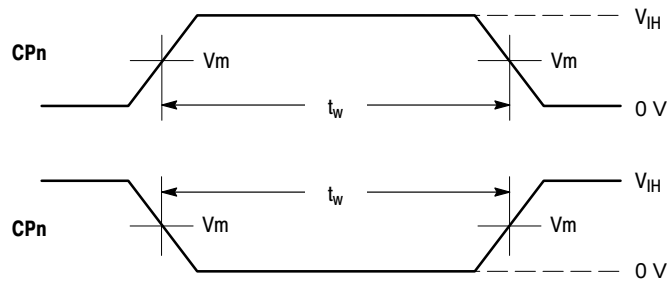
Figure 5. AC Waveforms
