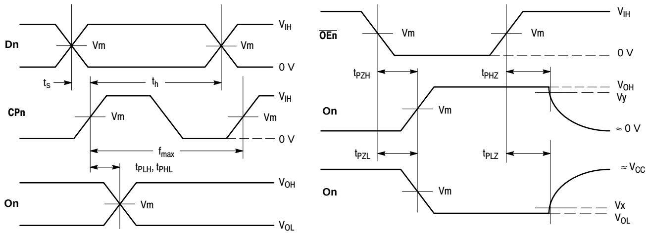
WAVEFORM 4 – PROPAGATION DELAYS, SETUP AND HOLD TIMES
