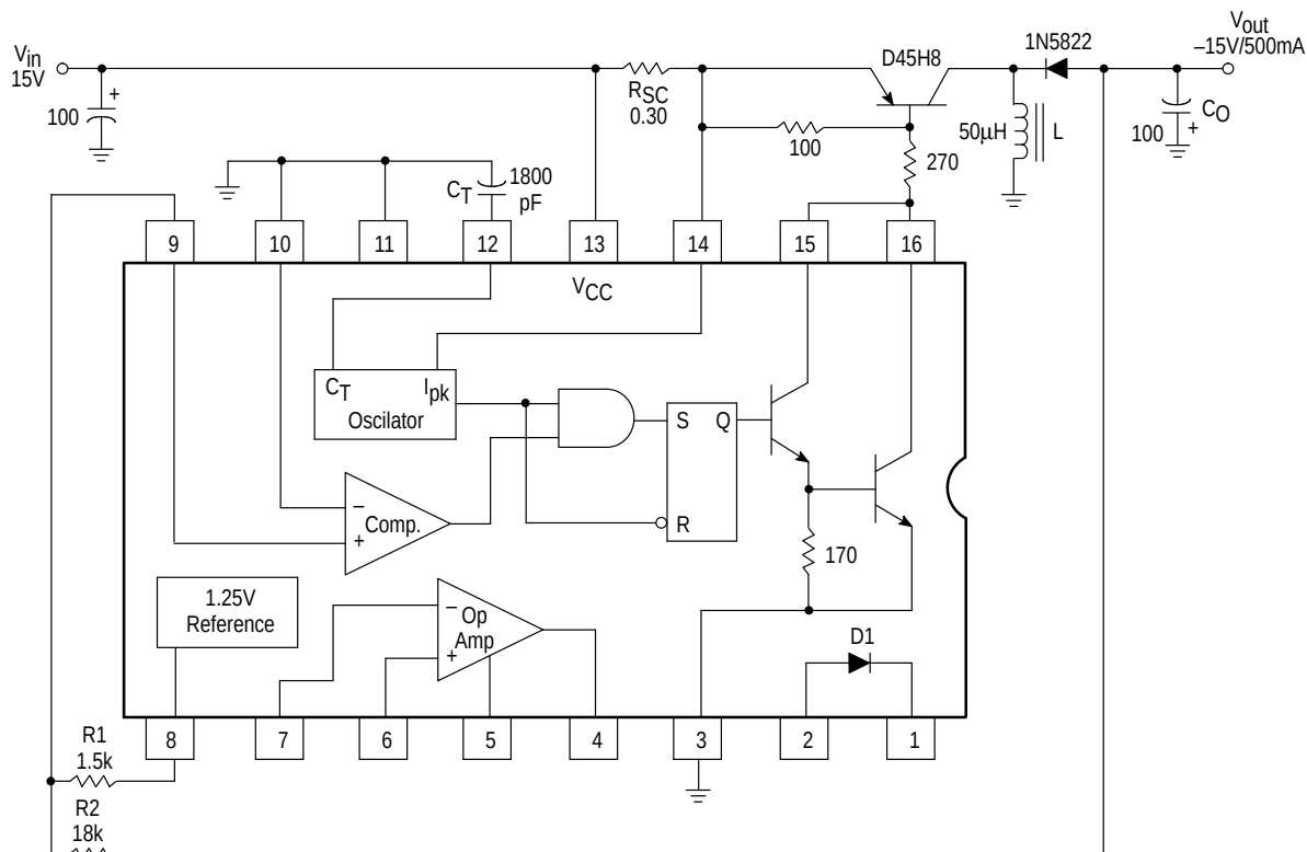
Figure 7. Inverting Converter
