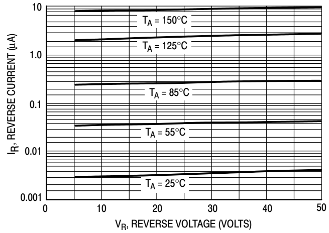
Figure 5. Leakage Current
