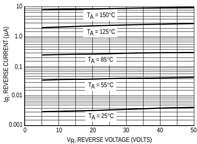
Figure 3. Leakage Current
