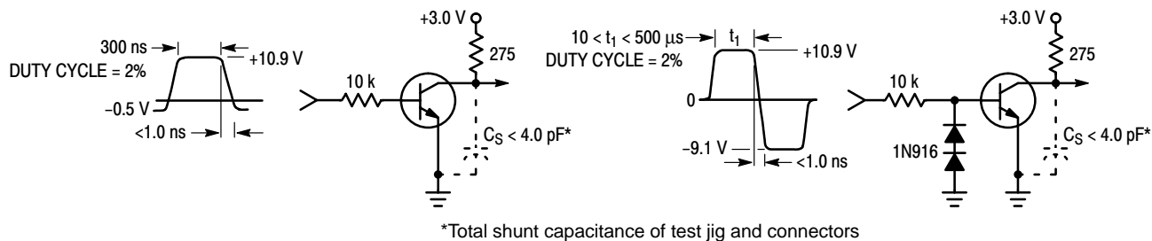
Figure 1. Turn–On Time
