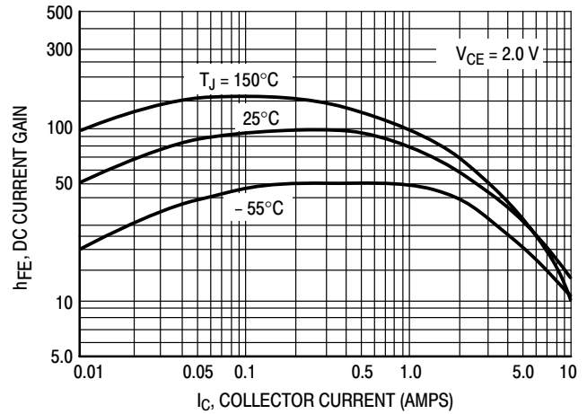
Figure 4. Current Gain
