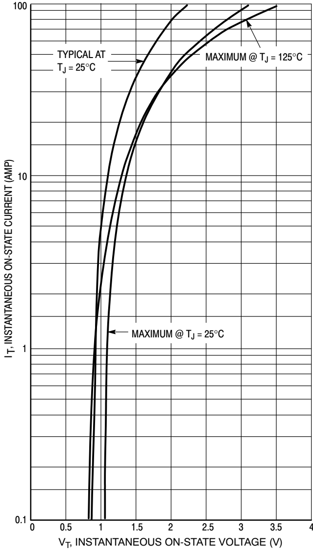
Figure 3. On-State Characteristics
