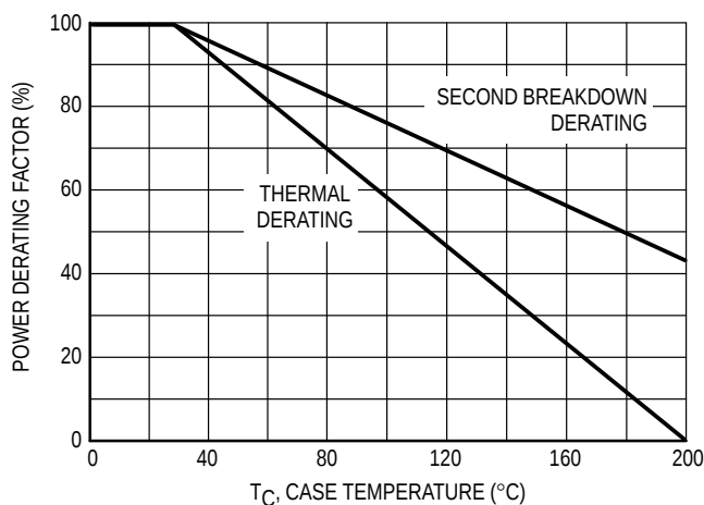
Figure 11. Power Derating
