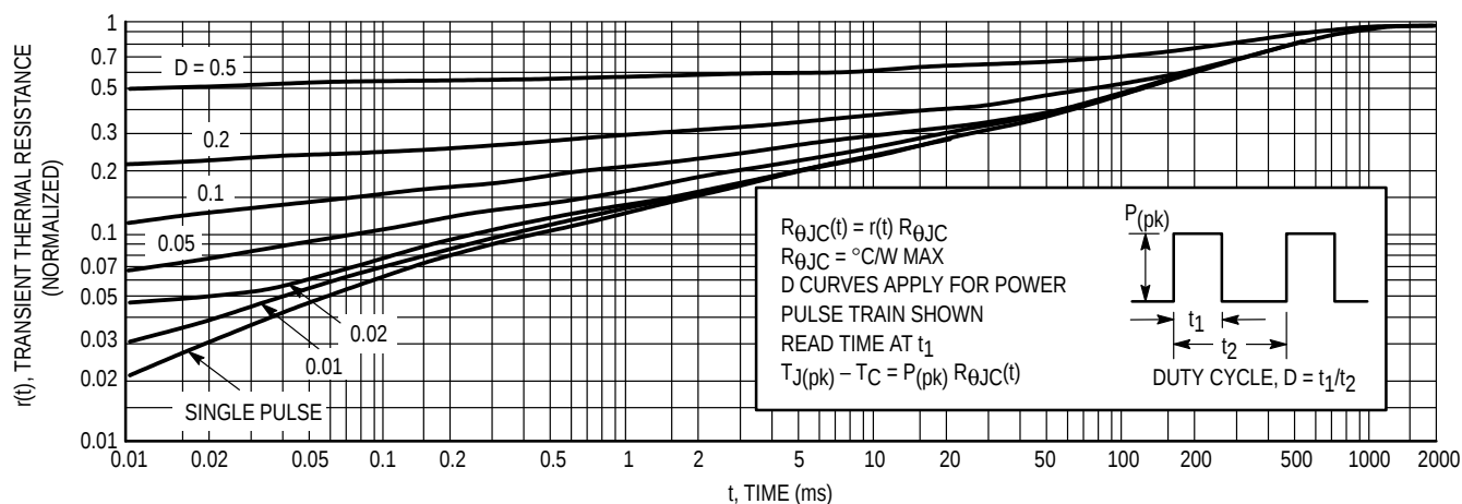
Figure 9. Thermal Response
