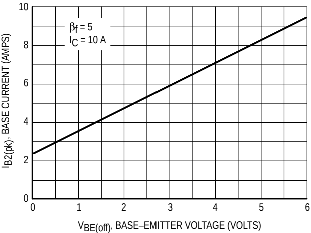
Figure 8. Peak-Reverse Current
