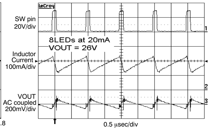
Figure 9. Switching Waveforms
