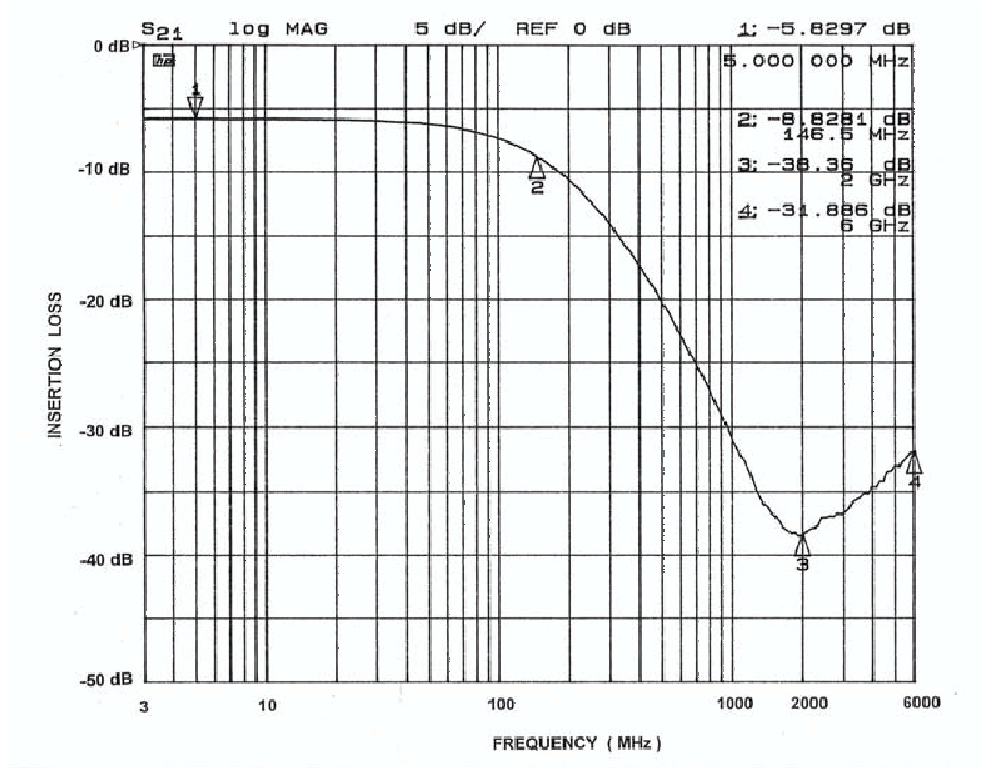
Figure 1. A1-C1 EMI Filter Performance
