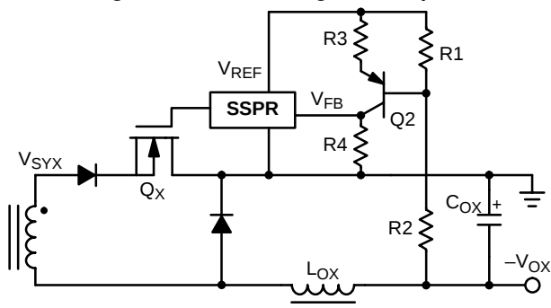
Figure 9. SSPR for Negative Output
