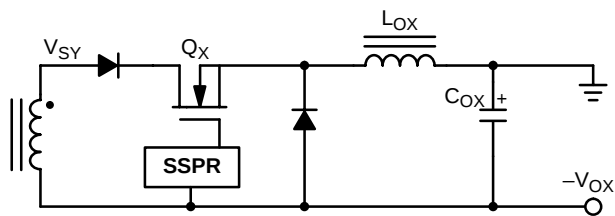
Figure 9. SSPR for Negative Output
