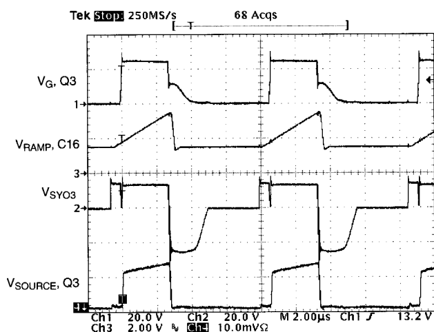
Figure 21. SSPR Waveforms
