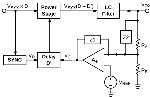
Figure 18. Modular Gain Block Diagram
