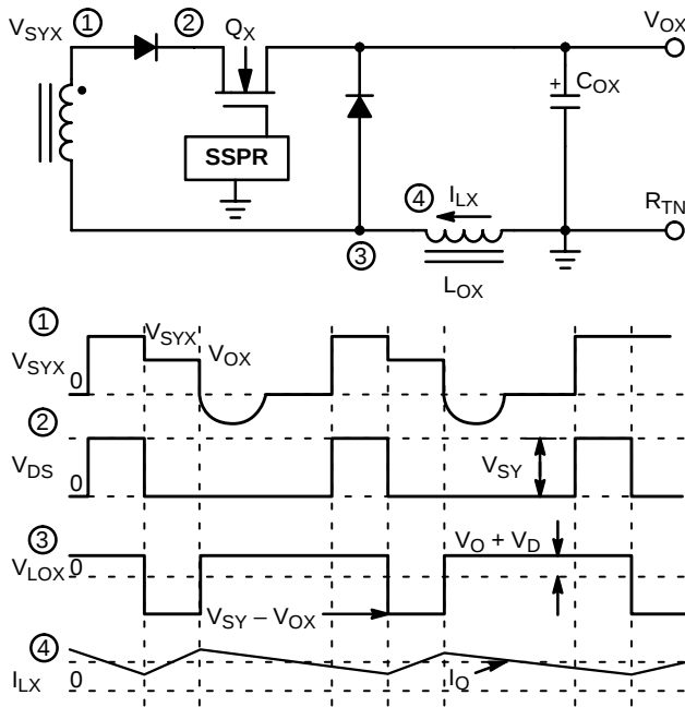
Figure 8. SSPR Connected in the Return
