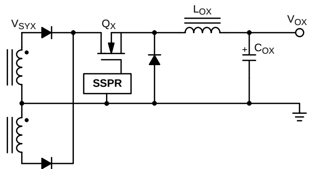
Figure 11. Dual Ended SSPR
