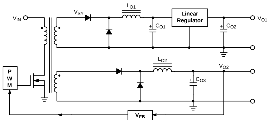
Figure 1. Linear Regulator
