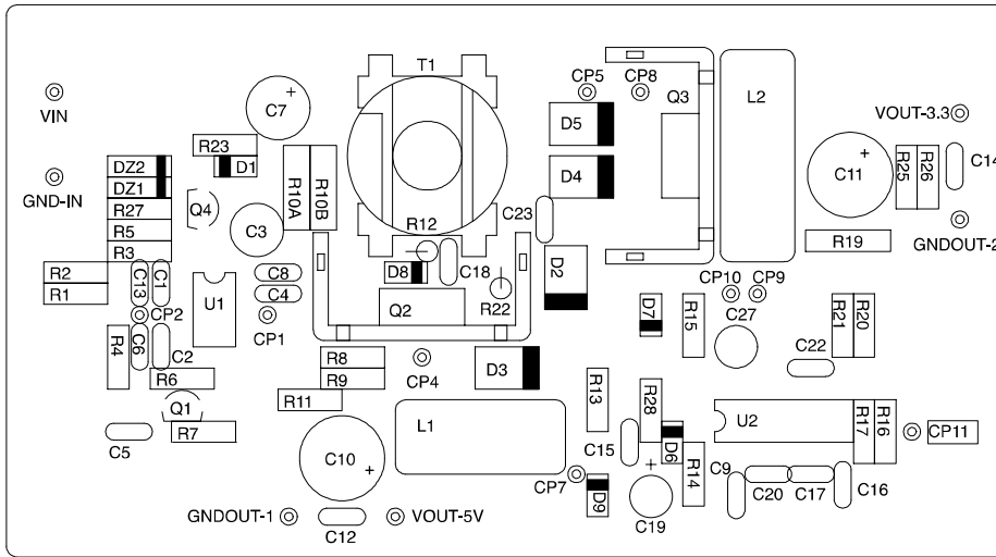
Figure 23. Component Placement
