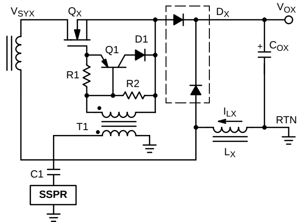
Figure 12. SSPR with Gate Drive Transformer
