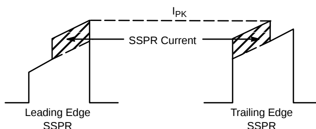
Figure 5. Primary Switch Current Waveforms
