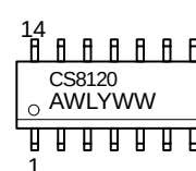
SO-14 D SUFFIX CASE 751A
