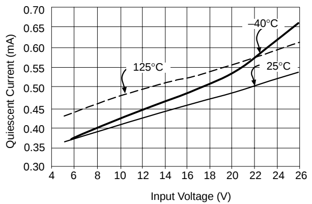
Figure 7. Quiescent Current vs. Input Voltage I_{OUT} = 100\text{ µA}
