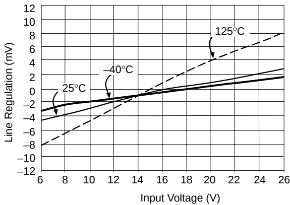
Figure 4. Line Regulation vs. Input Voltage I_{OUT} = 100\text{ µA}
