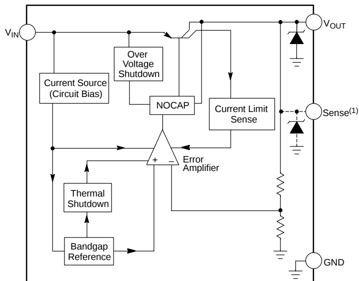
Figure 1. Block Diagram
