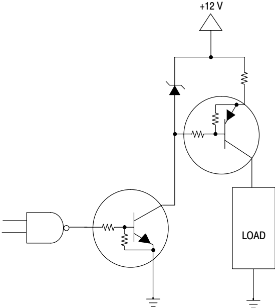
Figure 25. Inexpensive, Unregulated Current Source
