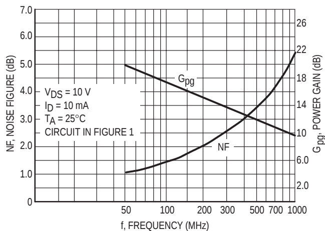
Figure 11. Noise Figure and Power Gain versus Frequency
