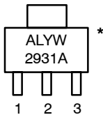
SOT-223 ST SUFFIX CASE 318H
