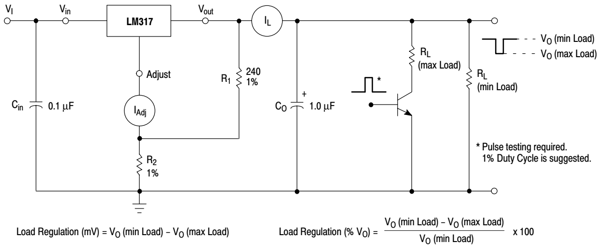
Figure 2. Load Regulation and \Delta I_{Adj}/\text{Load} Test Circuit
