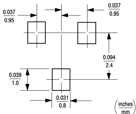
SC-59 POWER DISSIPATION
