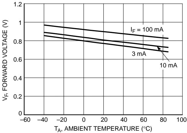
Figure 5. Forward Voltage versus Temperature
