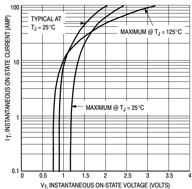
Figure 7. On-State Characteristics
