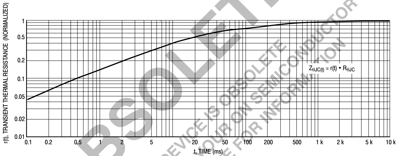
Figure 8. Thermal Response
